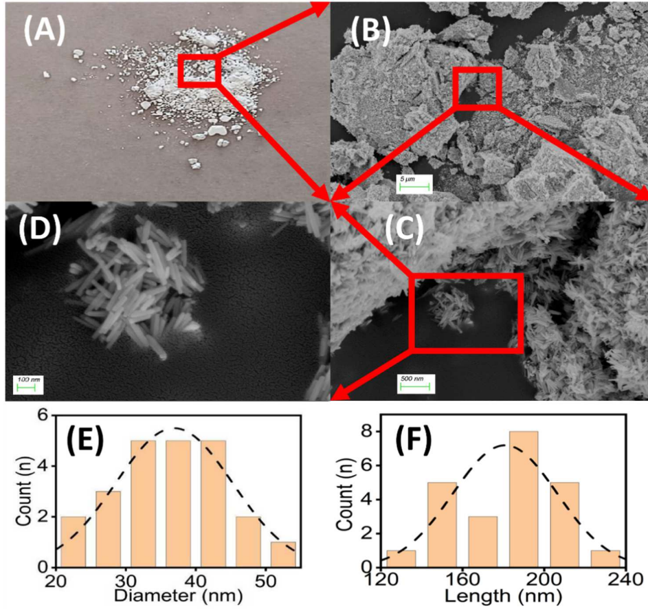
Fig. 2 (A) Optical image of ZnO nano rod powder. (B, C, D) SEM images of ZnO nano rods at 5K, 50K and 150K magnification respectively. (E,F) show the histogram plot of average diameter and length of ZnO nanorods.
