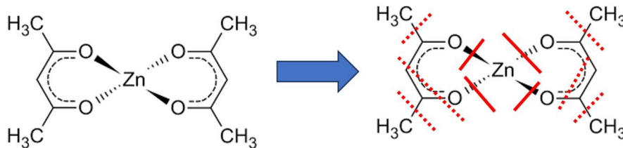
Fig. 9 Schematic diagram of breaking of zinc acetylacetonate.
