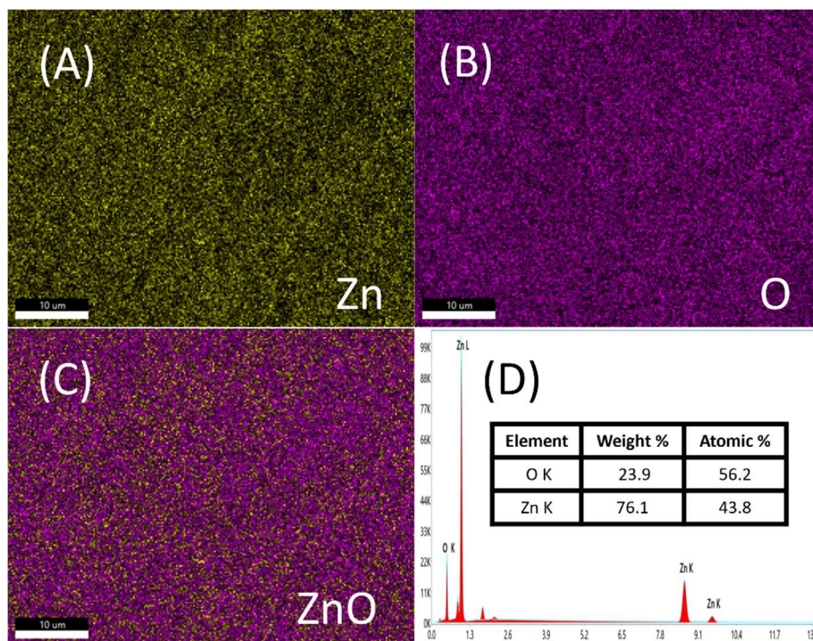
Fig. 4 Elemental mapping of (A) Zn, (B) O and (C) ZnO in ZnO nanorods. (D) EDAX of ZnO nanorods.
