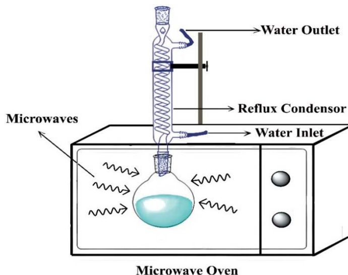
Fig. 1 Schematic diagram of microwave synthesis method setup.
