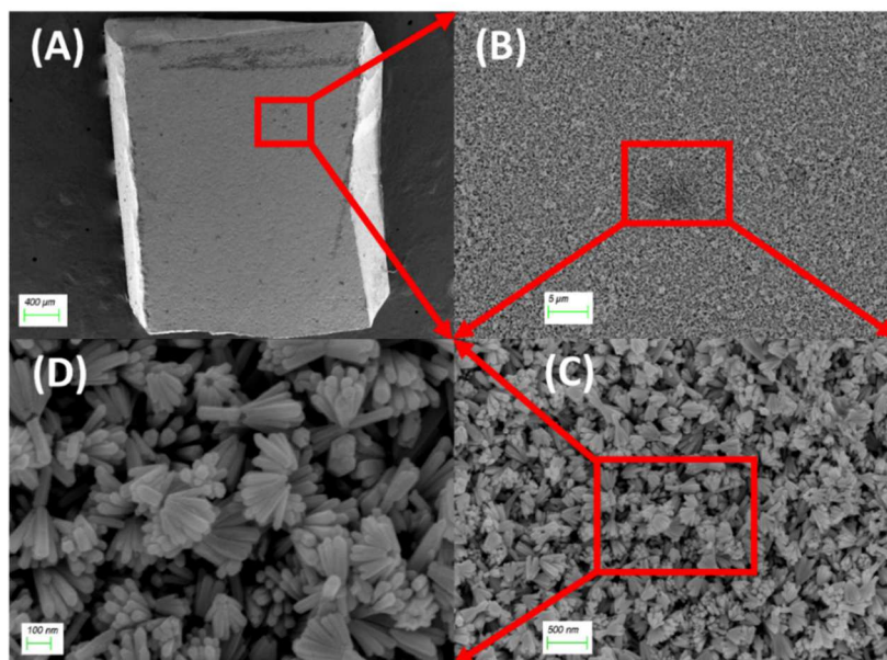
Fig. 3 (A) SEM image of ZnO nanorods growth on silicon (100) substrate viewed at 55X. (B, C, D) SEM images of ZnO nanorods at 5K, 50K and 150K magnification respectively.
