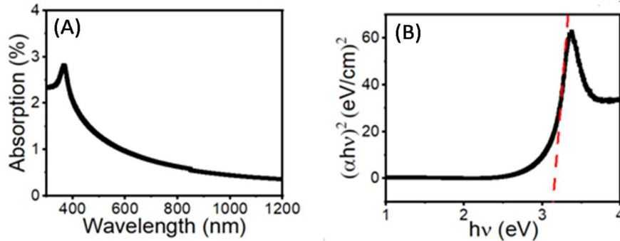
Fig. 6 UV visible spectra ZnO nanorods. (a) Absorption band (b) Tauc plot revealing the bandgap.
