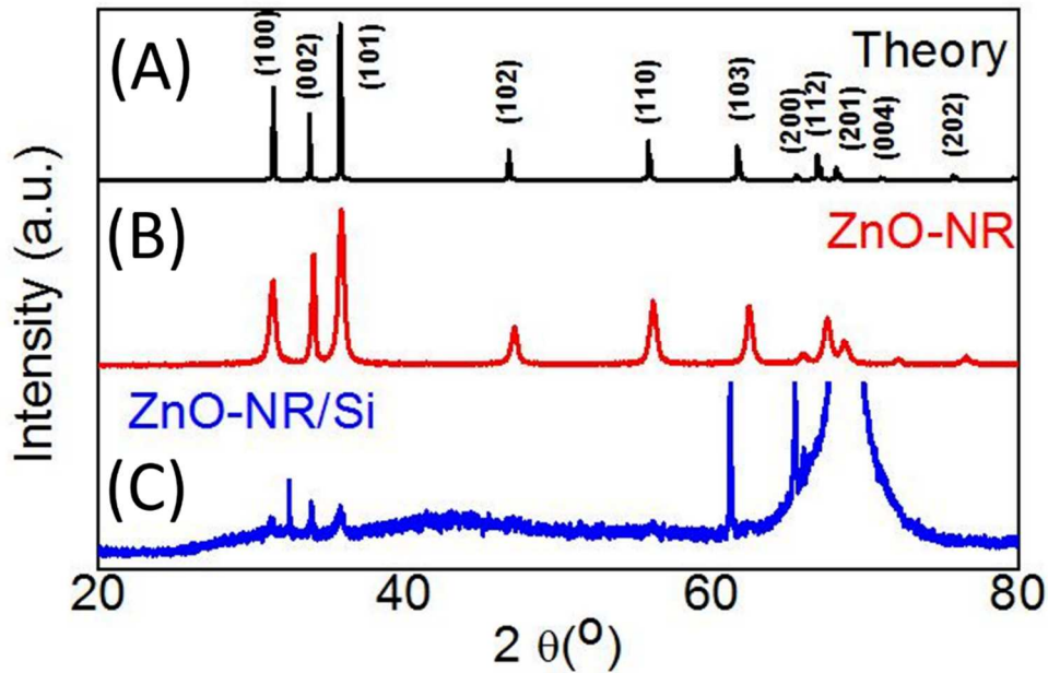
Fig. 5 XRD results of (A) theoretical wurtzite structure ZnO, (B) ZnO nanorods powder (C) ZnO nanorods grown on Si(100) substrate.
