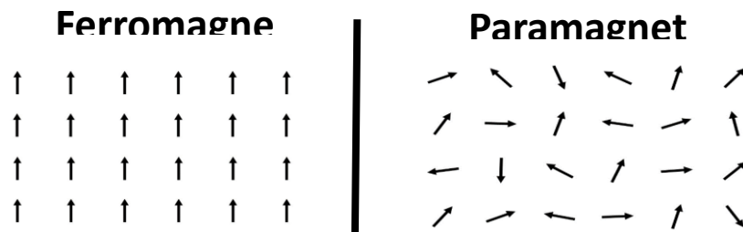
Fig.1.: Schematic illustration of spin arrangement for a ferromagnet (spin-order phase) and a paramagnet (spin-disorder phase). The arrows indicate the spin magnetic moment at each atomic site.
