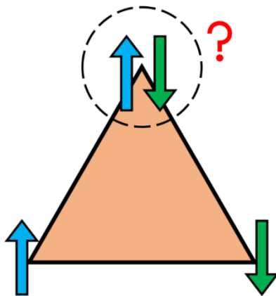
Fig..3. depicts frustration in an antiferromagnetic triangular lattice i.e. when one spin points upward and the other downward, the third spin remains in a state of confusion as it cannot satisfy both of them simultaneously since adjacent spins prefer to point in opposite directions because of antiferromagnetic constraint.
