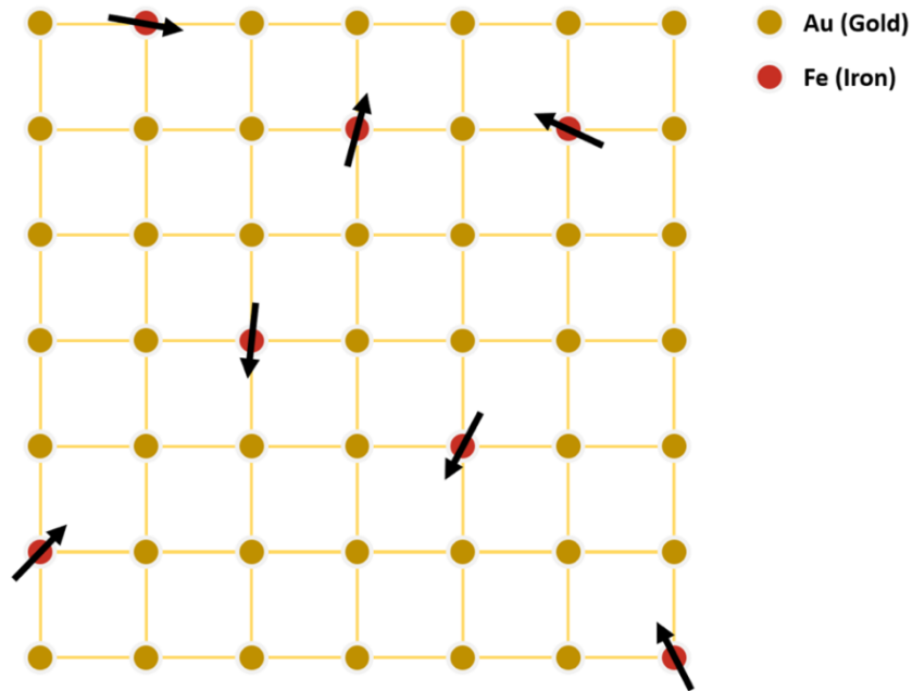
Fig..2. Schematic illustration of AuFe spin glass in which the iron atoms as magnetic impurities are mixed randomly to the nonmagnetic gold matrix. The spins associated with iron atoms represented by arrows are trapped in random directions.
