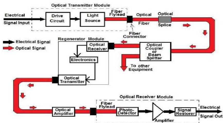
Fig. 2. Block Diagram
